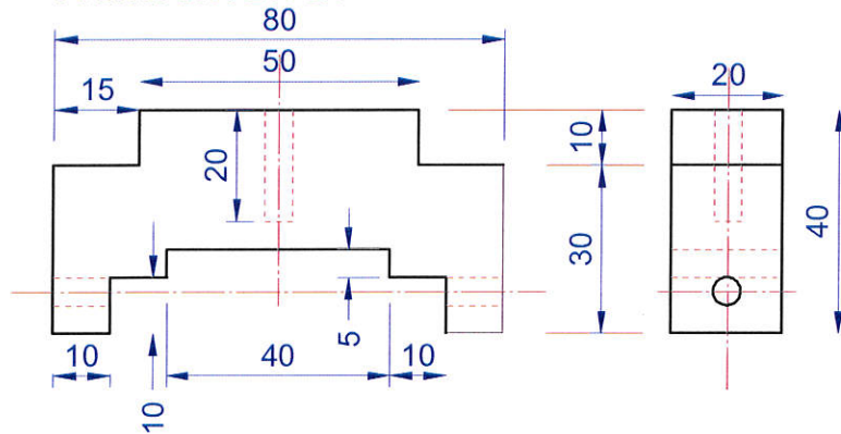
Front Axel Block
