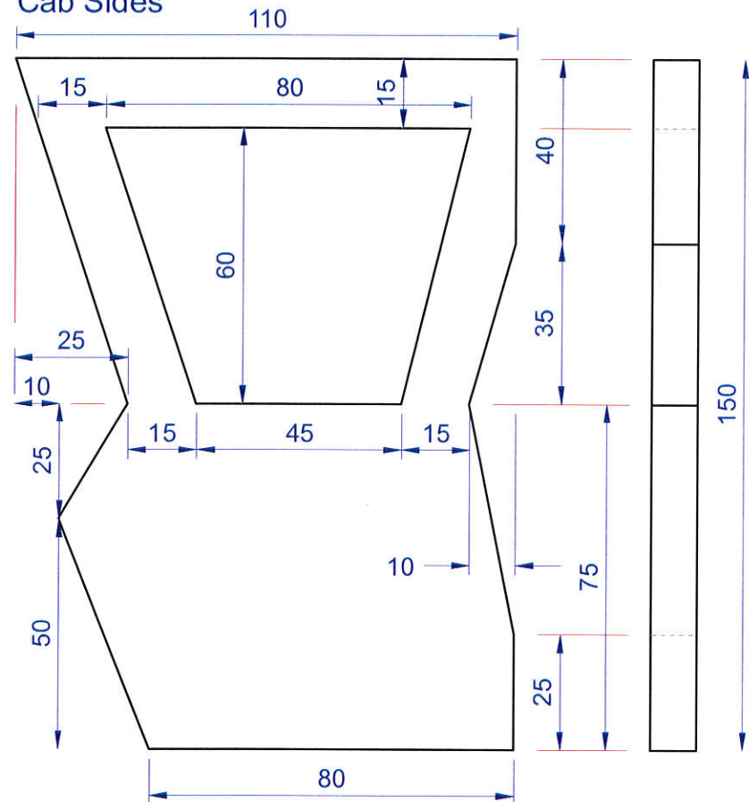
Cab Sides
